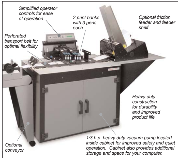
Conveyor, shelf and feeder, shown above, may vary from representation in size and color.
